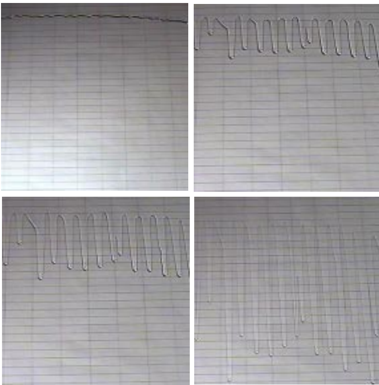
FIG. 1. Photos of the fluid flowing down an inclined plane at times = 0.5, 4, 8, 84 sec after release (increasing from top left to bottom right). The inclination angle is \alpha = 60^\circ ; other fluid and flow parameters are given in §3. The distance between the solid lines is 5 cm in the transverse, and 2 cm in the downhill direction.
