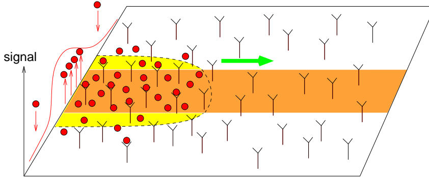
Figure 1: The schematics of switching on of an autocrine loop in a row of cells expressing a ligand-processing protease. The ligand is secreted only in a narrow strip of the epithelium, but is degraded upon binding to receptors which are uniformly distributed throughout the epithelium. The pattern is initiated by a localized input at the left end of the epithelium and propagates to the right. The dashed line shows an instantaneous level set of the ligand concentration at the cell surfaces.
