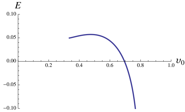
Figure 3: The energy E of the bounded positive solutions as a function of \nu_0 for \nu = 2 and a = 0.4 .
