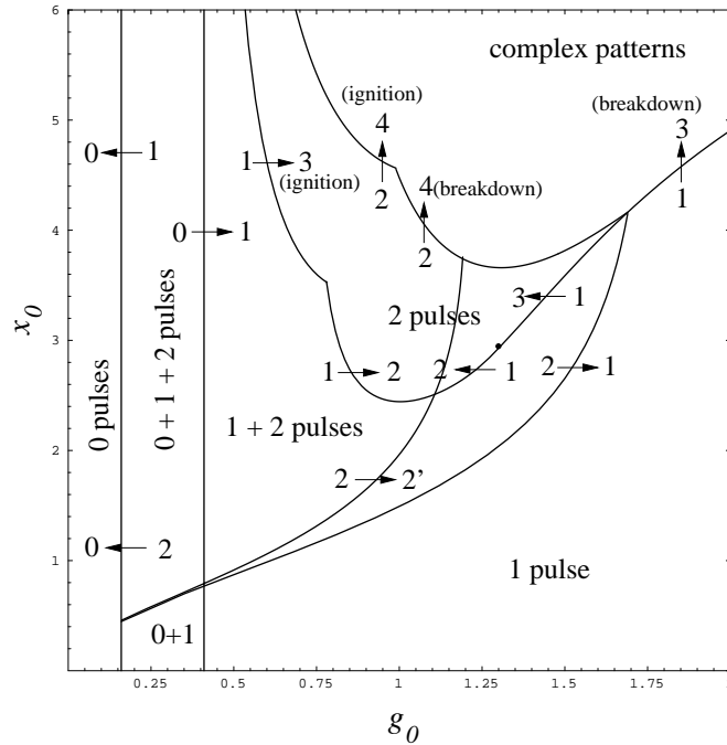
Fig. 5. Multiple steady states and transitions between them as functions of the inductive signal's width and amplitude. The network parameters are: b_r = 0.2 , c_r = 0.4 , \lambda = 1.6 .
