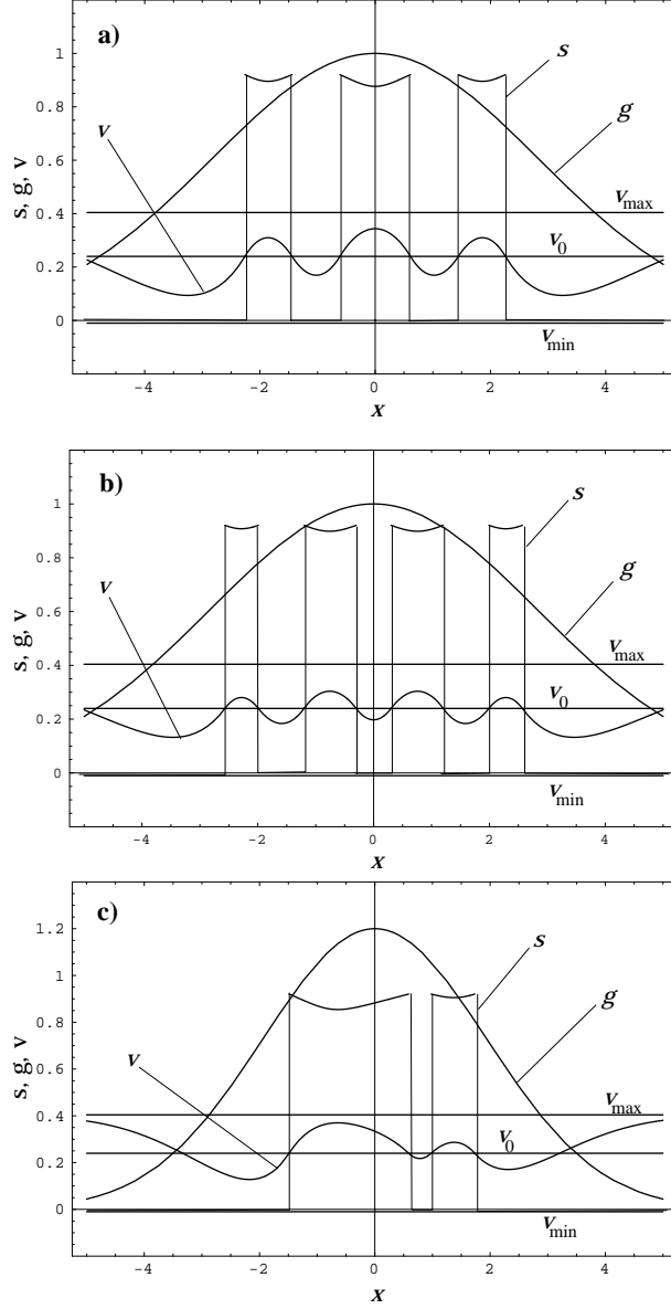
Fig. 4. Asymptotic solutions in the form of complex signaling patterns. The parameters are as in Fig. 3, except: x_0 = 4, g_0 = 1 in (a) and (b), x_0 = 2.75, g_0 = 1.2 in (c).
