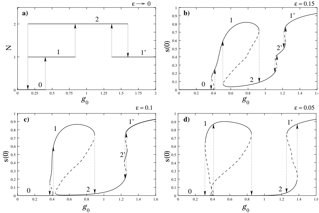
Fig. 6. (a) The sequence of transitions upon the adiabatic variation of the inductive signal's amplitude. (b) – (d) One parameter bifurcation cuts showing the value of s in the center of the system in the stationary solutions of the full model and transitions between them [Eqs. (5) – (8)]. The parameters are as in Fig. 2, except \epsilon = 0.15 (b), \epsilon = 0.1 (c), and \epsilon = 0.05 (d). N in (a) is the number of pulses; numbers in (b) – (d) indicate different stationary solutions with the corresponding number of peaks, solid lines show stable, and dashed lines — unstable solutions.
