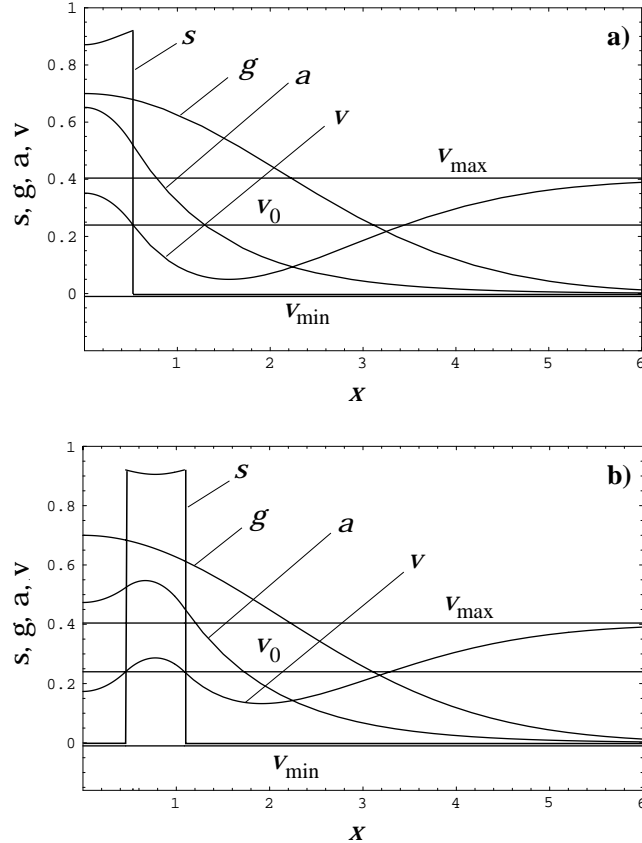
Fig. 3. Asymptotic one and two pulse solutions (only half of the solution is shown). The parameters are: b_r = 0.2 , c_r = 0.4 , \lambda = 1.6 , g_0 = 0.7 , x_0 = 3 .
