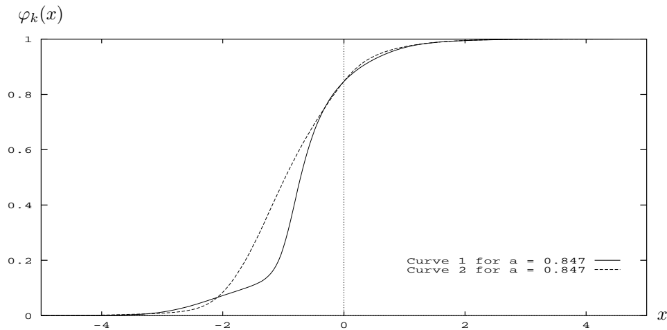
FIG. 3. Example 1: A solution plot for the period two pair of diffusion coefficients \alpha = 1.3, 1.9 .
