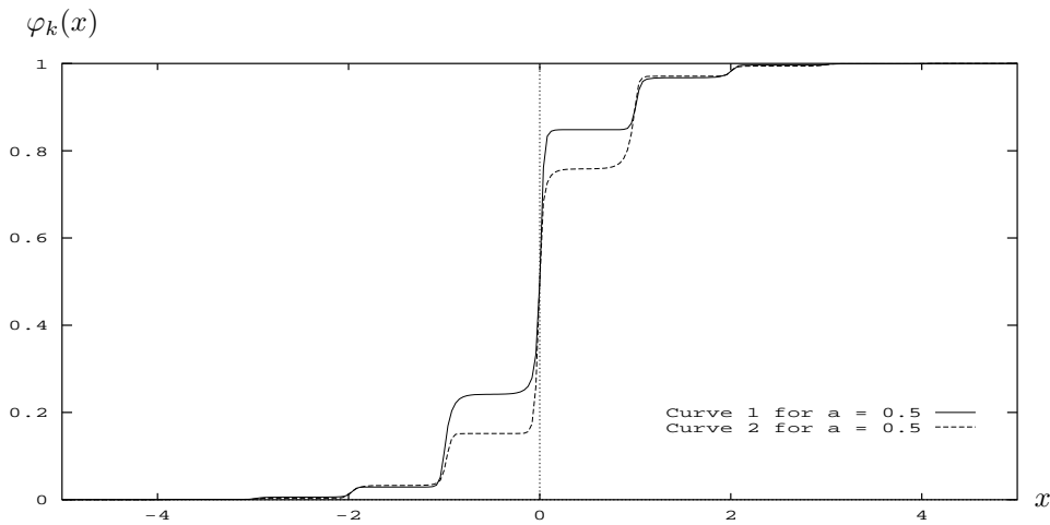
FIG. 8. Example 1: A solution plot for the period two pair of diffusion coefficients \alpha = 1.3, 1.9 .
