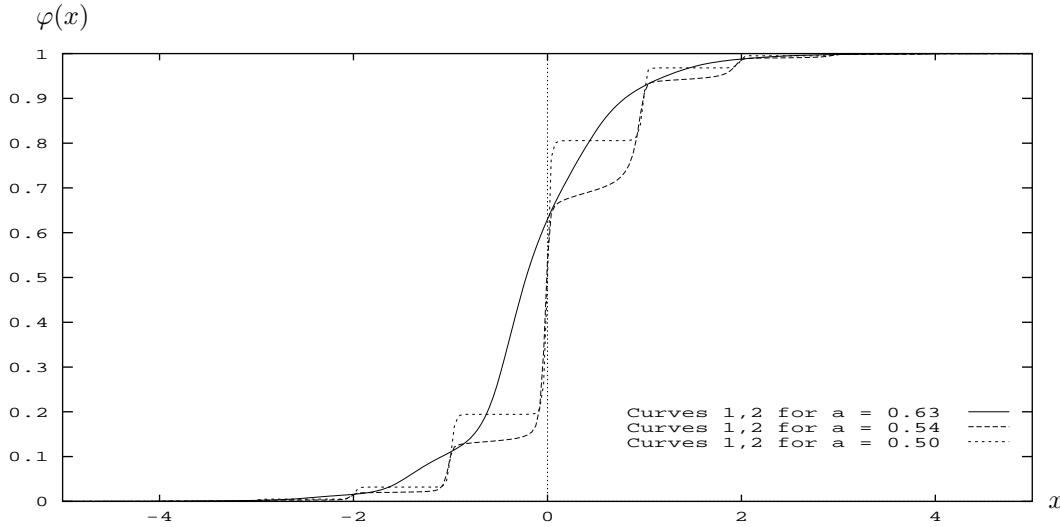
FIG. 13. Example 2: Constant diffusion coefficients. No period splitting.
