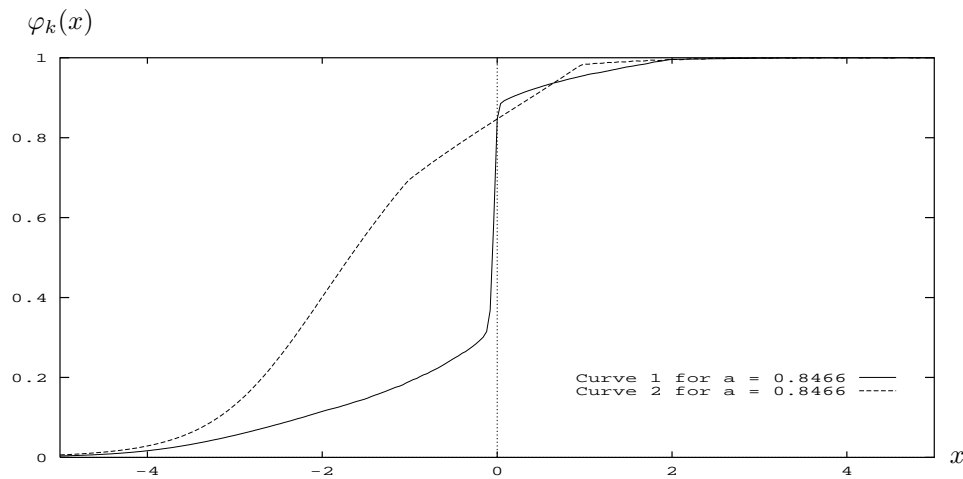
FIG. 4. Example 1: A solution plot for the period two pair of diffusion coefficients \alpha = 1.3, 1.9 .
