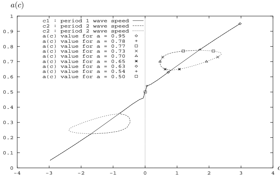
FIG. 9. Example 2: An a(c) plot for a constant coefficient problem.
