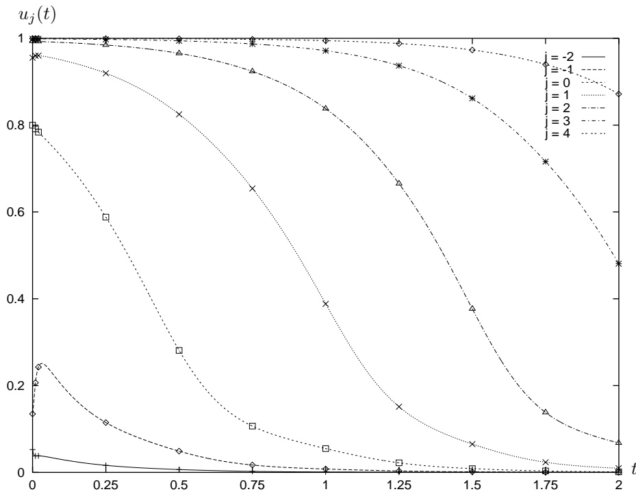
FIG. 25. The u_j versus t plot for a = 0.8 .
