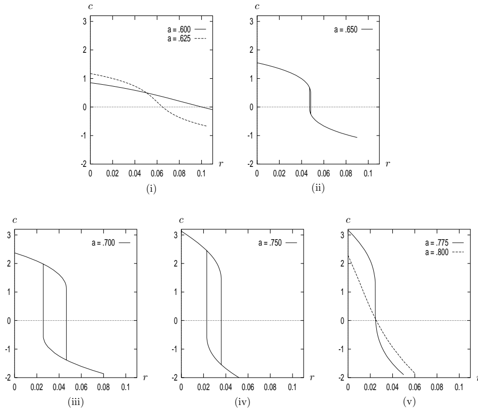
FIG. 19. Phase portrait: c(t) = c_e(t) - c_o(t) , the difference in wave speed, versus r(t) = r_e - r_o = \int_0^t c(s)ds , the phase shift.
