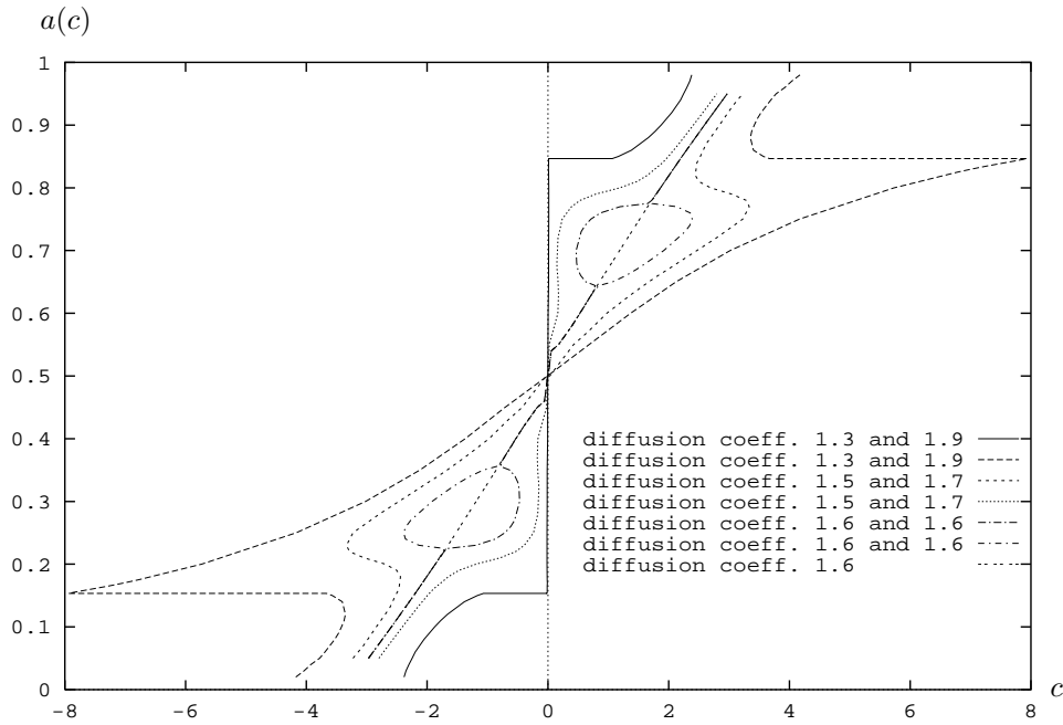
FIG. 14. A plot of a(c) curves for various choices of period 2 diffusion coefficients. The average of each pair of coefficients is 1.6. The a(c) curves appear in pairs.
