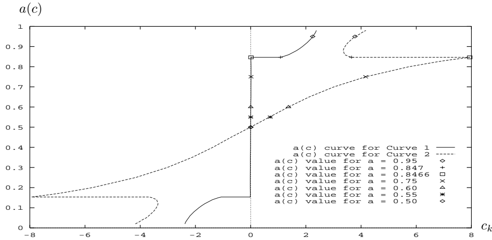
FIG. 1. Example 1: An a(c) plot for the period two pair of diffusion coefficients \alpha = 1.3, 1.9 .
