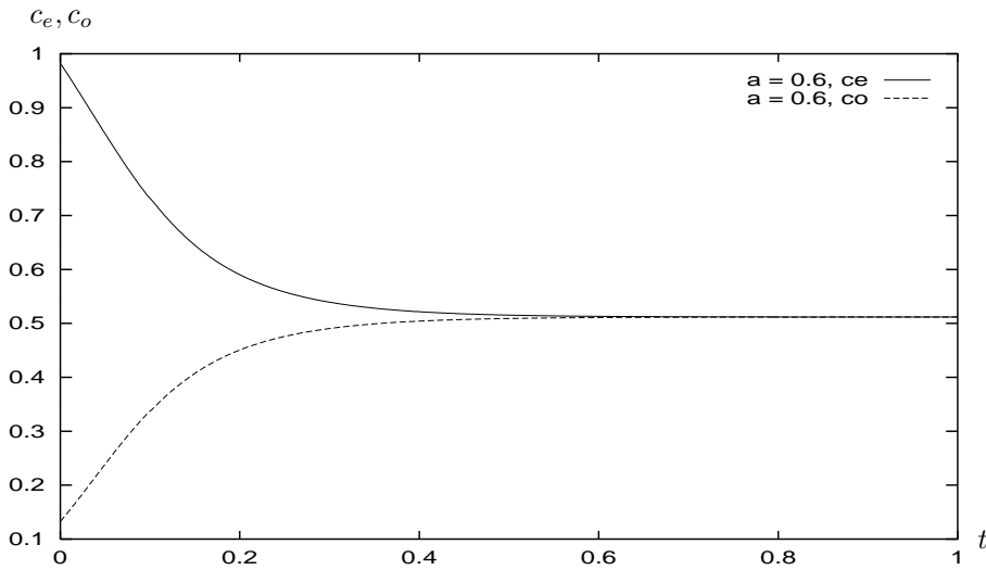
FIG. 23. The c_e(t), c_o(t) plot for a = 0.6 .
