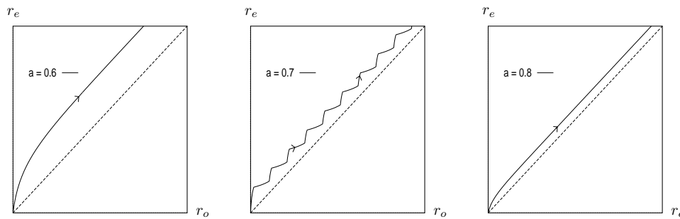
FIG. 20. Phase portraits of r_e = \int_0^t c_e(s)ds versus r_o = \int_0^t c_o(s)ds showing the flow with respect to time.
