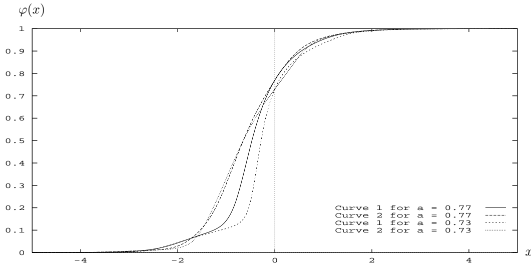
FIG. 11. Example 2: Constant diffusion coefficients. Period splitting.
