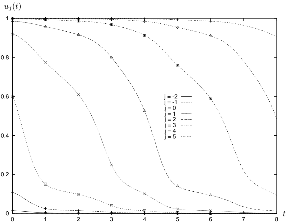
FIG. 22. The u_j versus t plot for a = 0.6 .
