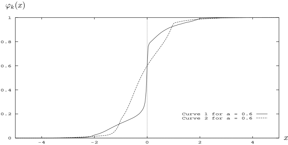
FIG. 6. Example 1: A solution plot for the period two pair of diffusion coefficients \alpha = 1.3, 1.9 .
