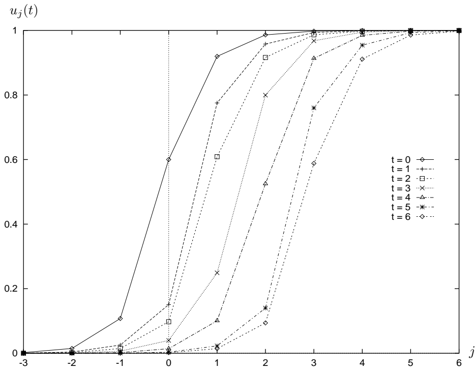
FIG. 21. The u_j versus j plot for a = 0.6 .
