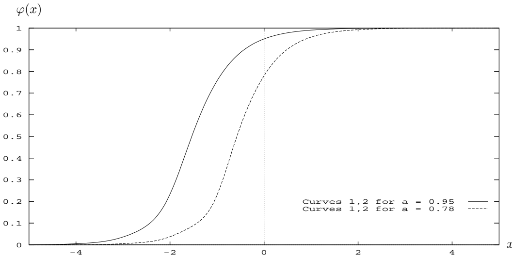
FIG. 10. Example 2: Constant diffusion coefficients. No period splitting.
