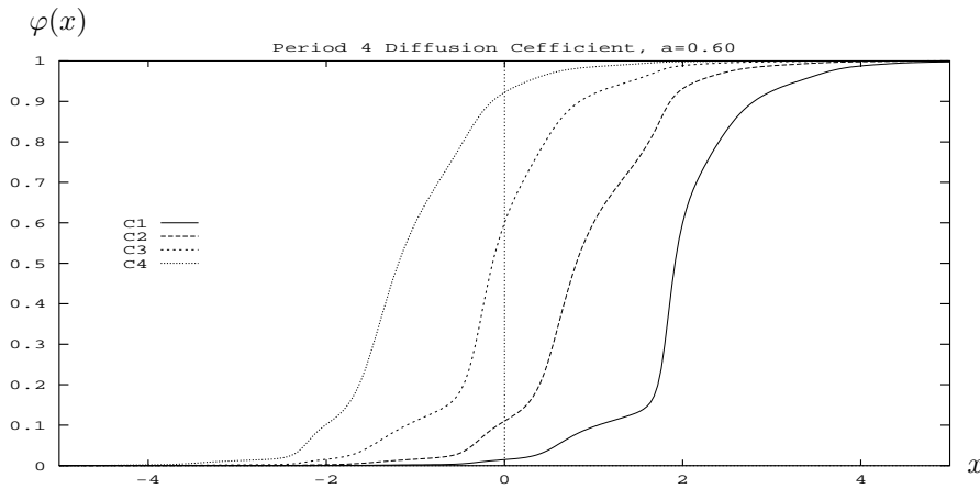
FIG. 17. Example 3: A solution plot for the period four diffusion coefficients \alpha = 1.4, 1.5, 1.6, 1.7 .
