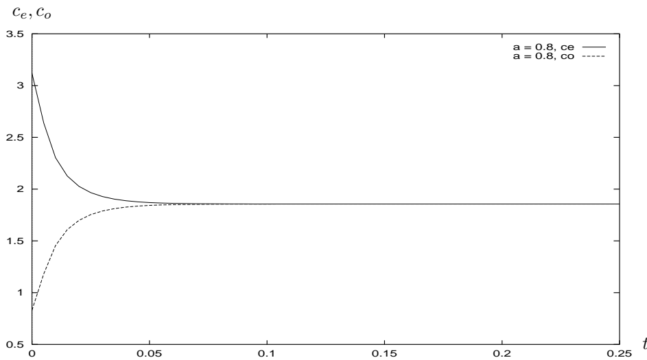
FIG. 26. The c_e(t), c_o(t) plot for a = 0.8 .
