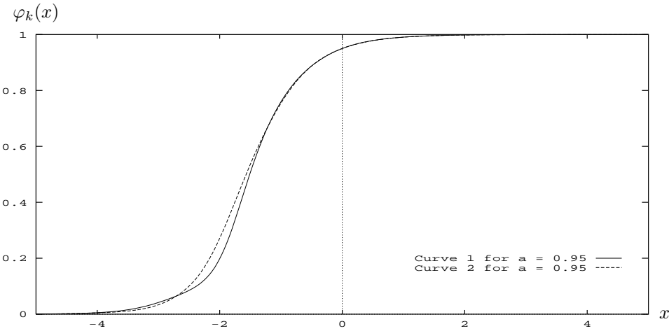
FIG. 2. Example 1: A solution plot for the period two pair of diffusion coefficients \alpha = 1.3, 1.9 .
