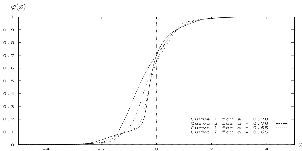
FIG. 12. Example 2: Constant diffusion coefficients. Period splitting.
