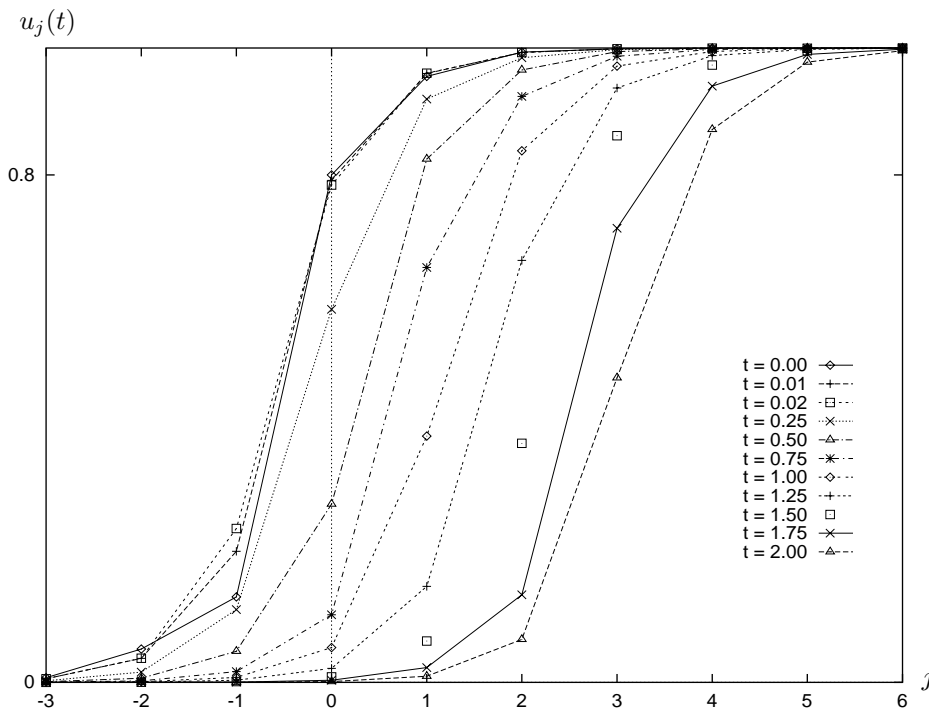
FIG. 24. The u_j versus j plot for a = 0.8 .
